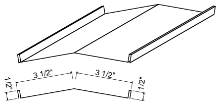
RIDGE / HIP
