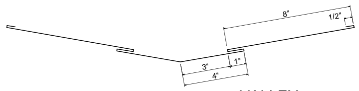
VALLEY
